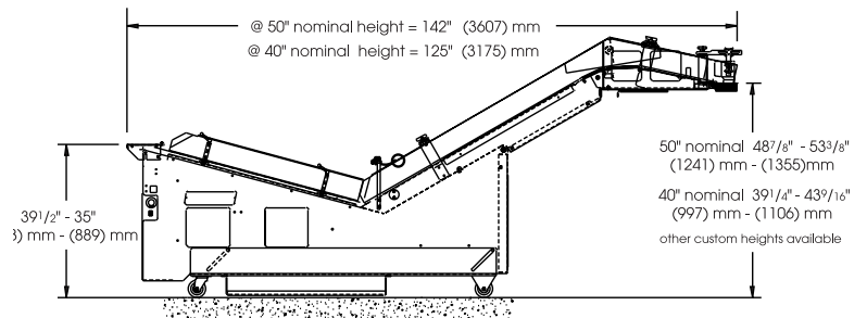
Three belts designed into quick adjustment rear "tail" taper and head-tail jogger. Scales provided for quick make-ready.
