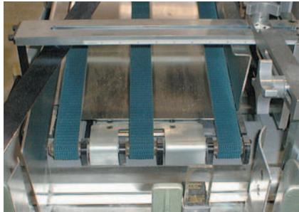
Three belts designed into quick adjustment rear "tail" taper and head-tail jogger. Scales provided for quick make-ready.
