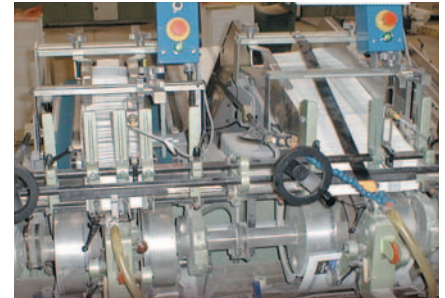
Capabilities to handle the narrow card stock as well as signature sizes are shown here.
